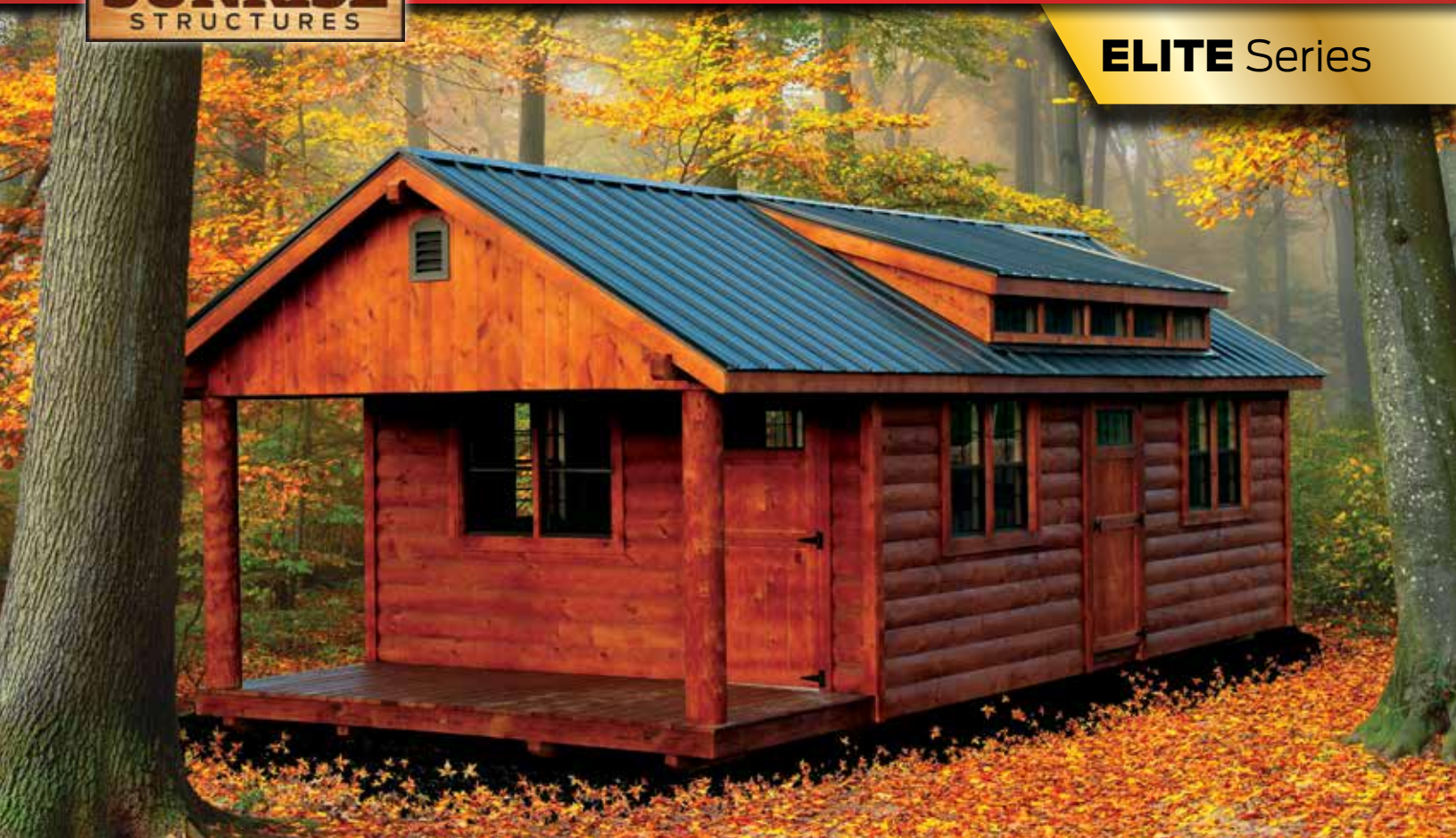
14' x 34' Elite Series Gable Cabin rustic cedar stain, burnished slate metal roof. Options include a 14' roof dormer, 3' transom door with brown window, log edition corbels and eight 2' x 3' brown windows.
